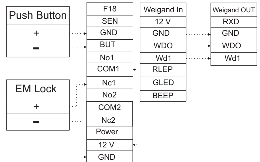
F18 with KR 500 & EM Lock Connection
